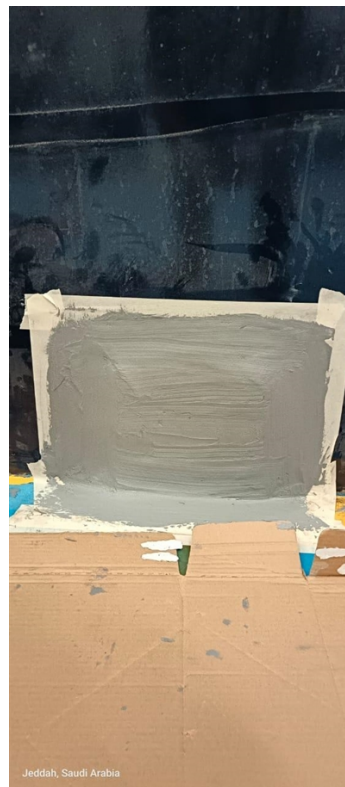
Plate bonding application using Belzona 1111 (Super Metal)
