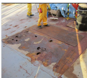
Holes in the surface plate of the deck due to severe corrosion
