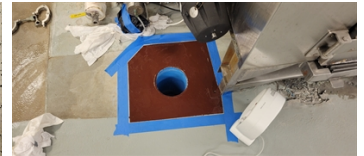
Second drain, application with Belzona 4311
