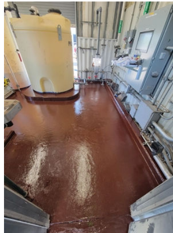
Application of second coat of Belzona 4311 red
