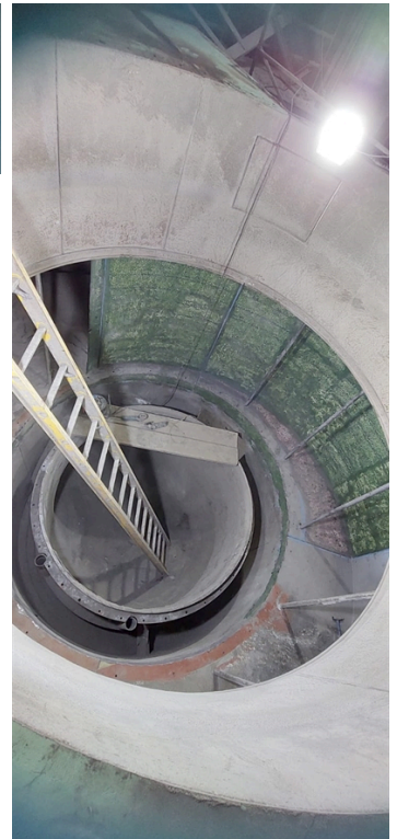
Application completed after applying Belzona 9811 then grouted with Belzona 1813
