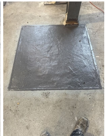
Repair completed with a final coat of Belzona 4311 to encapsulate the aggregate.
