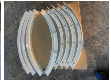
Second coat of Belzona 1331 applied and final product.
