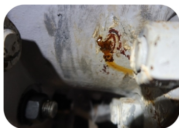
Damage on valve caused by corrosion and pipe aging
