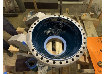
Belzona 2141 applied as a topcoat to protect against future cavitation damage
