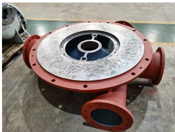
Pump efficiency improved with Belzona 1341 (Supermetalglide)
