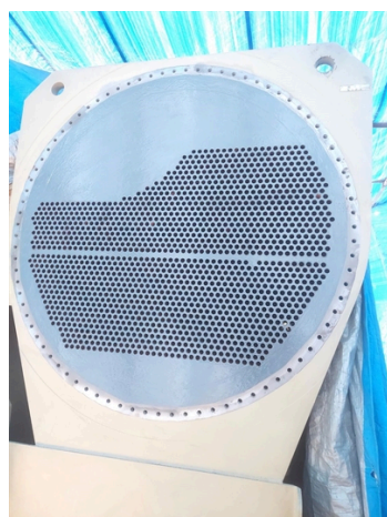
Chiller after Belzona 1321 and Belzona 1341 applications.
