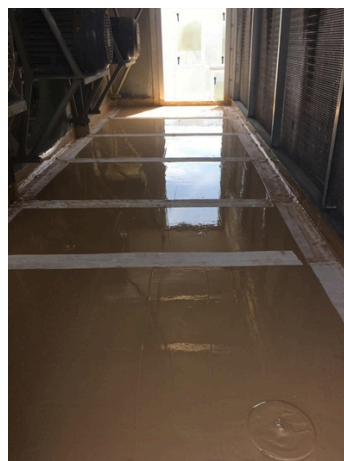
First coat of Belzona 5831 applied with Belzona 9341 Reinforcement Sheet over the seams.
