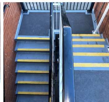
Stairwells repaired, a low slip coating added with Belzona Granogrip step edgings and all brickwork sealed with Belzona 5122 clear cladding
