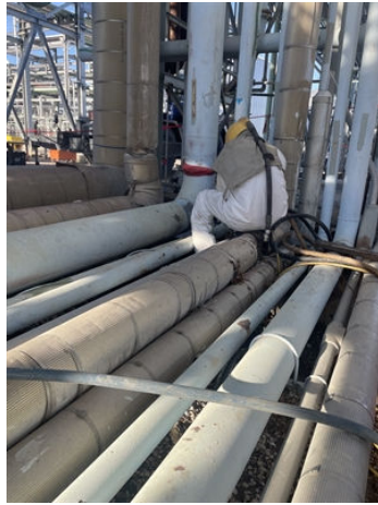
Application of Belzona 1161.
