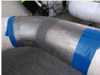
Surface preparation and weld seam rebuilt with Belzona 1212 E Metal
