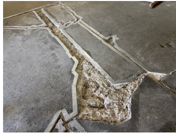
Grinding out of defective areas
