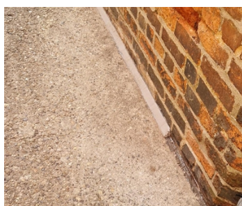
Flaunch applied at 35mm 45 degrees slope to ensure there is no square edge termination point to the Belzona 3131
